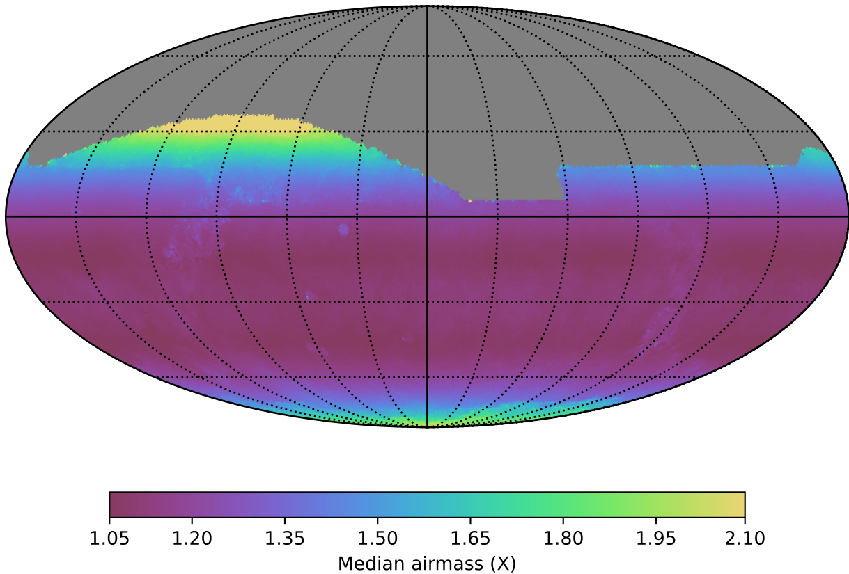
noroll_v3.4_10yrs All sky i band: Median airmass
