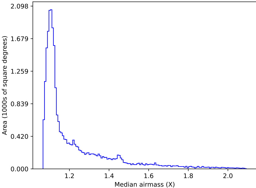
noroll_v3.4_10yrs All sky i band: Median airmass
