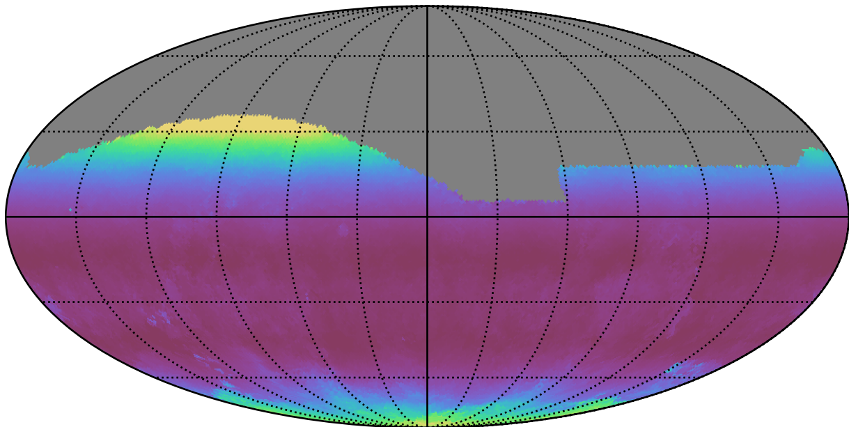
noroll_v3.4_10yrs All sky g band: Median airmass
