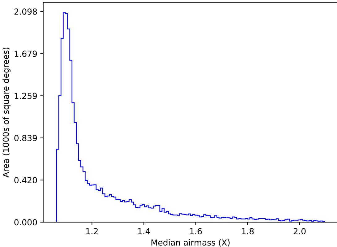
noroll_v3.4_10yrs All sky g band: Median airmass
