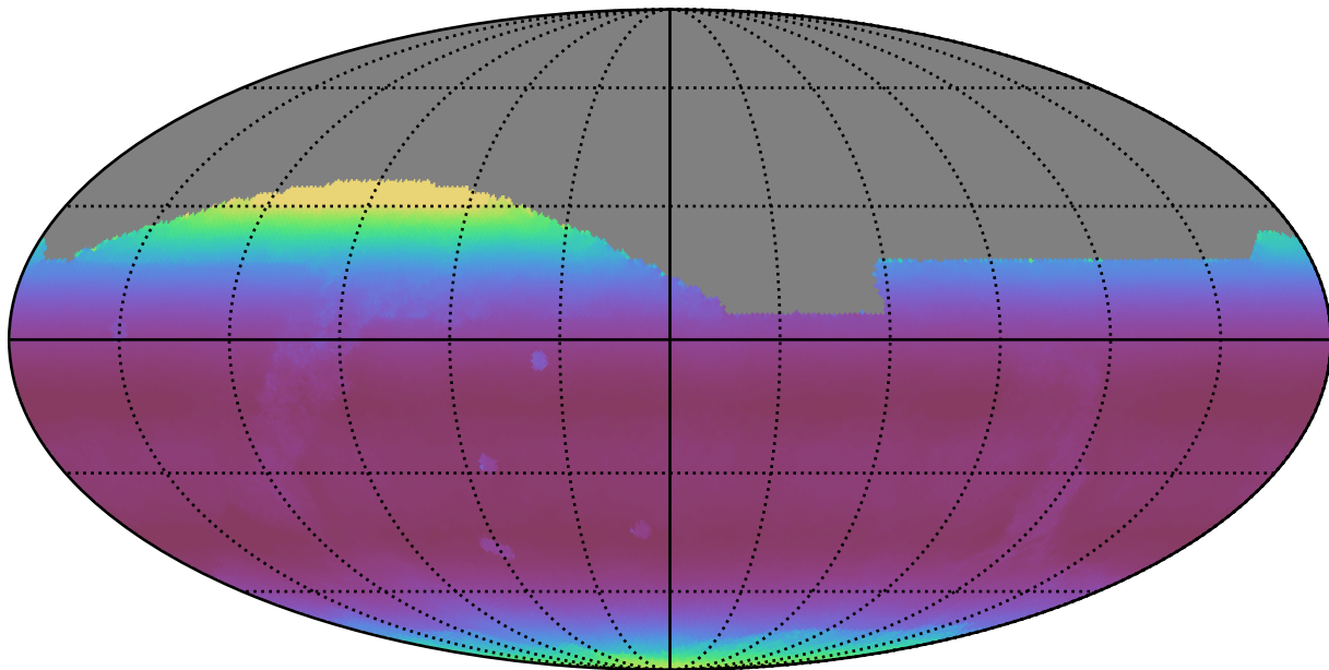
noroll_v3.4_10yrs All sky all bands: Median airmass
