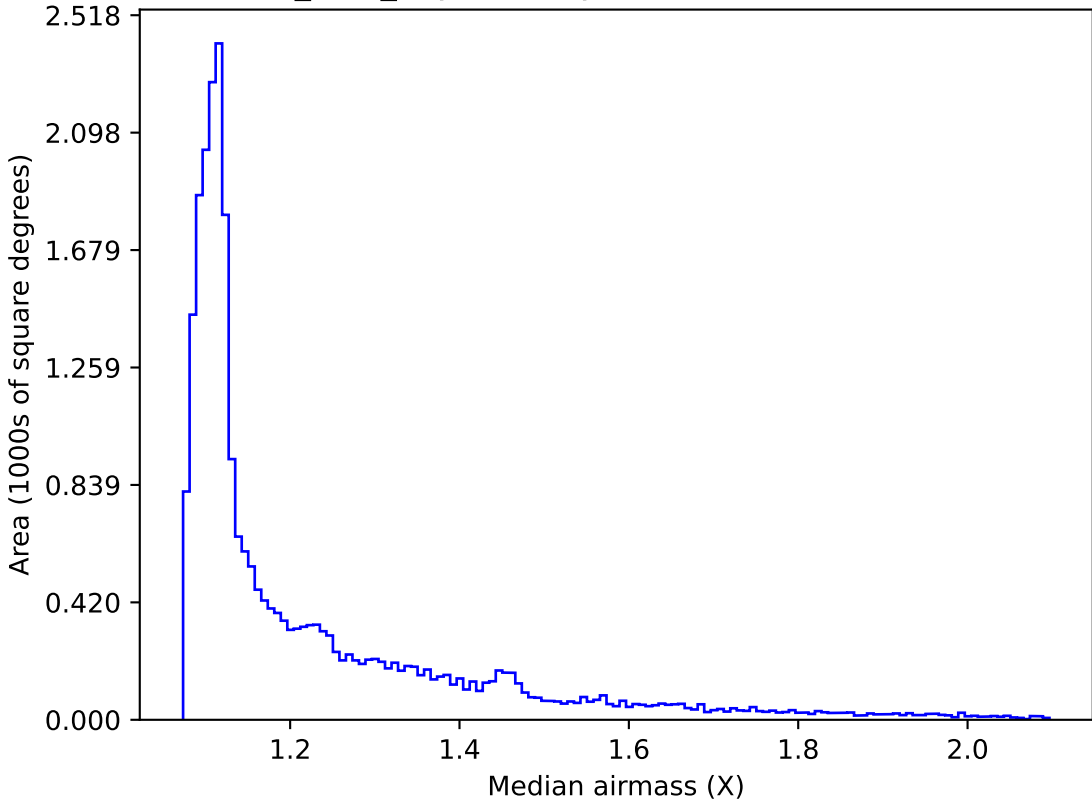
noroll_v3.4_10yrs All sky all bands: Median airmass
