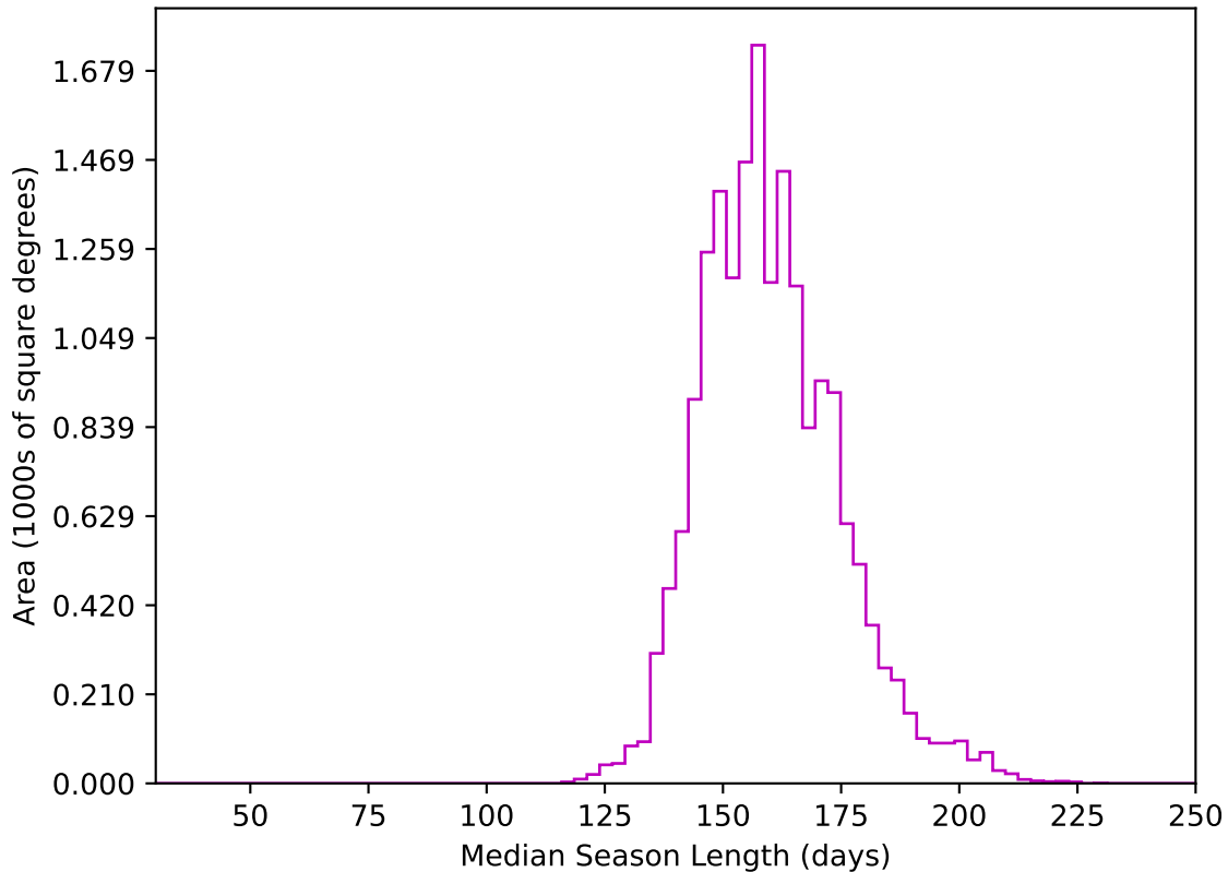
noroll_v3.4_10yrs WFD z band: Median Season Length
