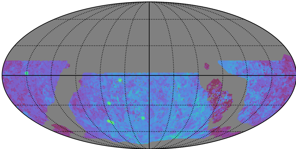
noroll_v3.4_10yrs WFD u band: Median Season Length
