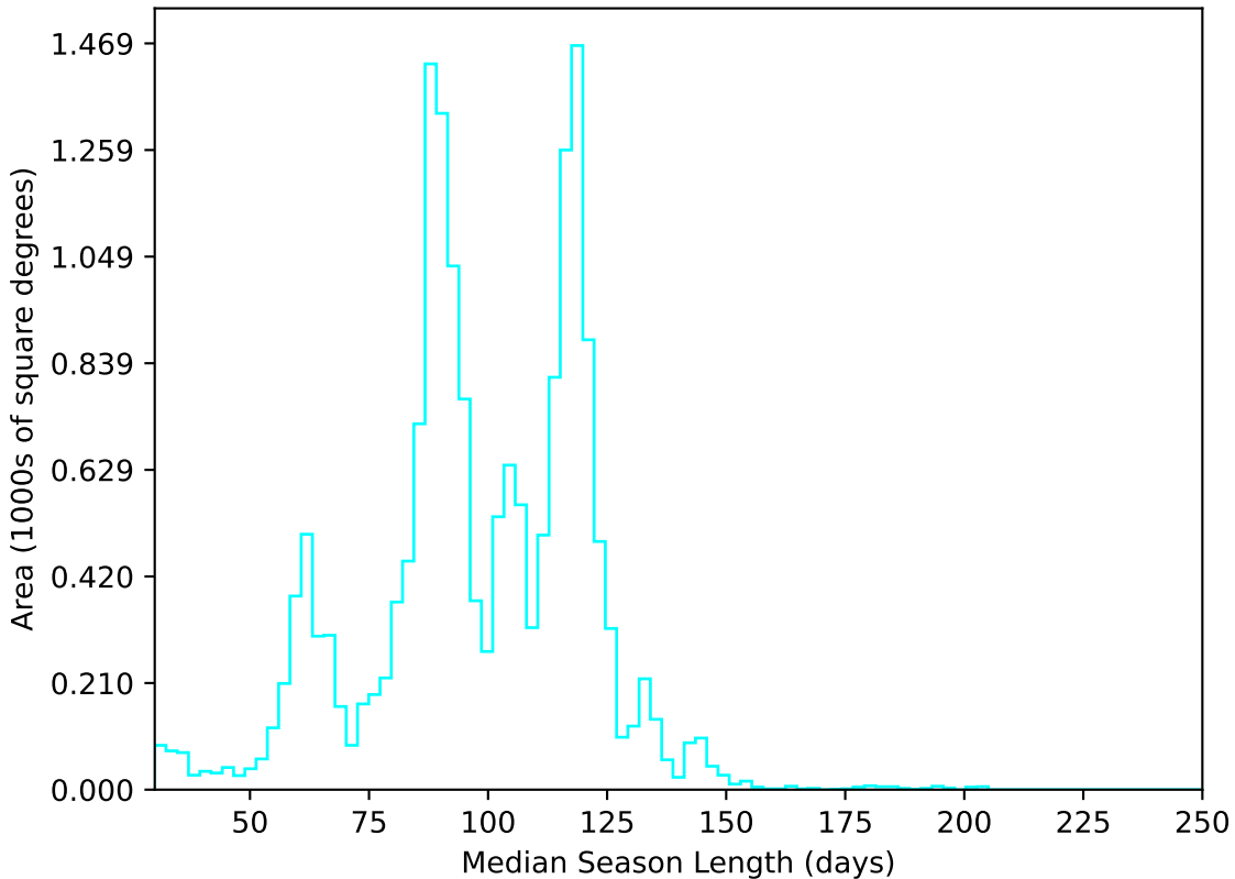
noroll_v3.4_10yrs WFD u band: Median Season Length
