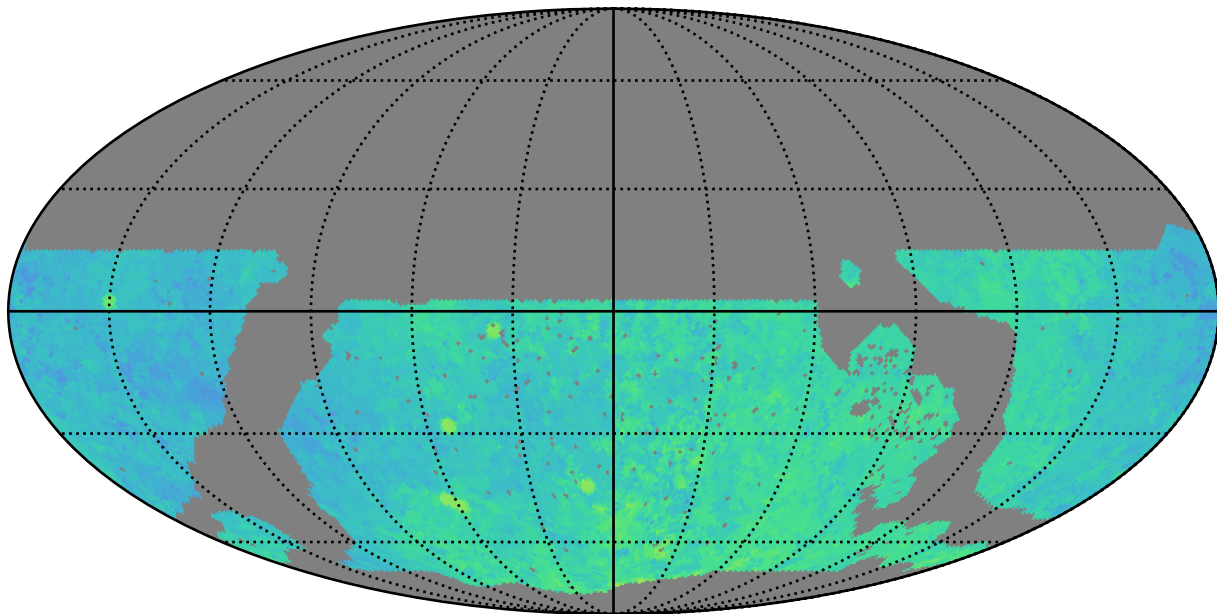
noroll_v3.4_10yrs WFD r band: Median Season Length
