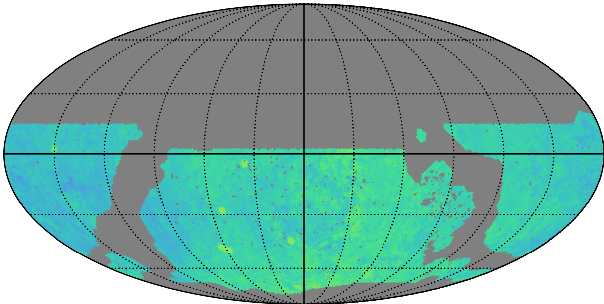
noroll_v3.4_10yrs WFD i band: Median Season Length
