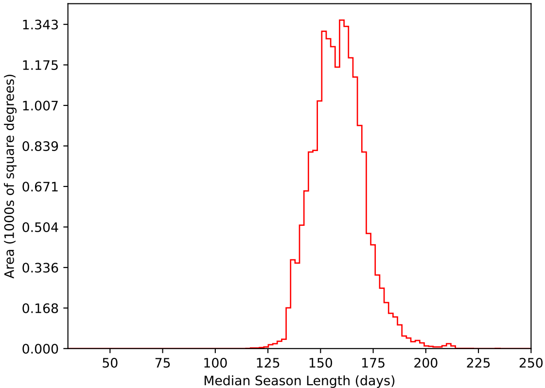
noroll_v3.4_10yrs WFD i band: Median Season Length
