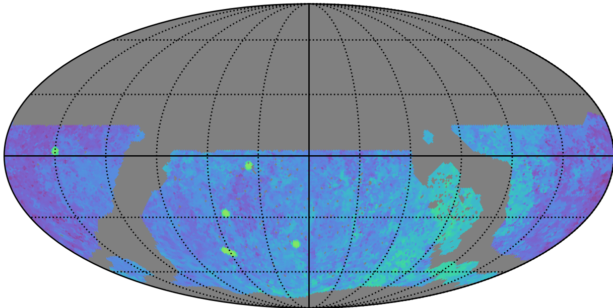
noroll_v3.4_10yrs WFD g band: Median Season Length
