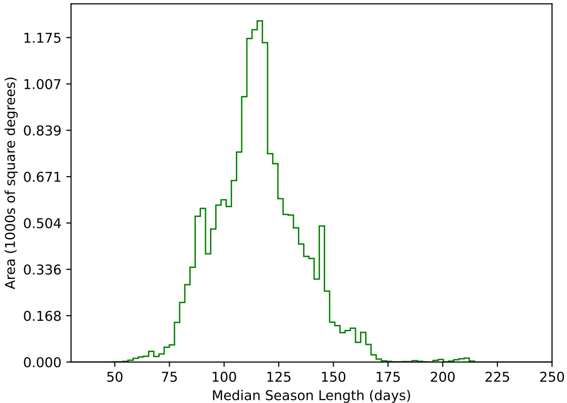
noroll_v3.4_10yrs WFD g band: Median Season Length
