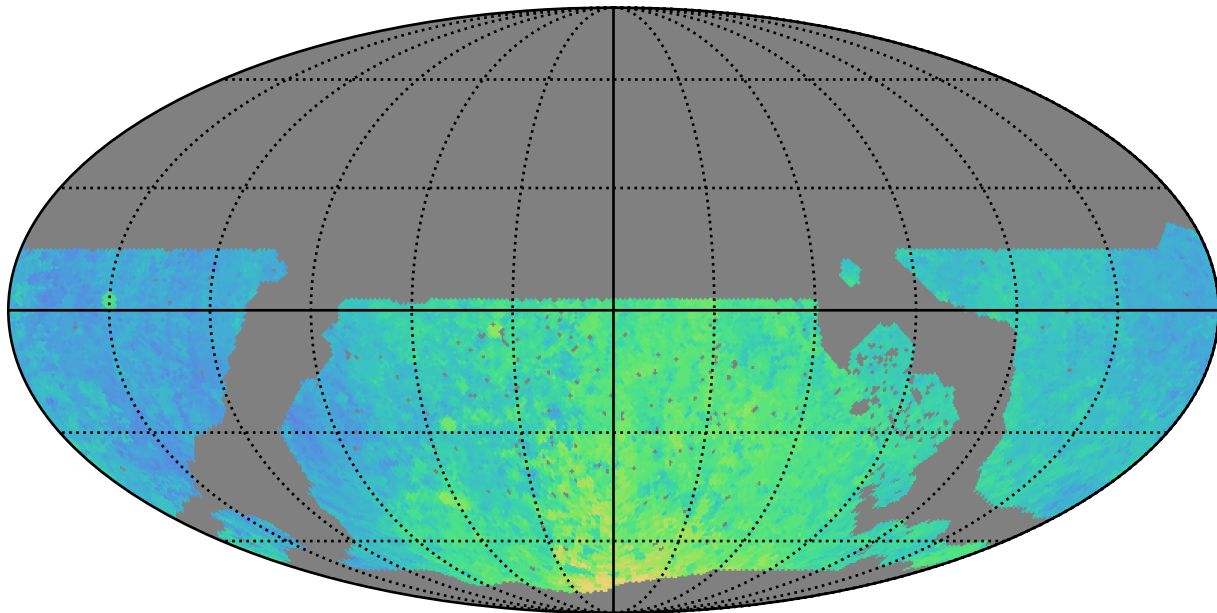
noroll_v3.4_10yrs WFD all bands: Median Season Length
