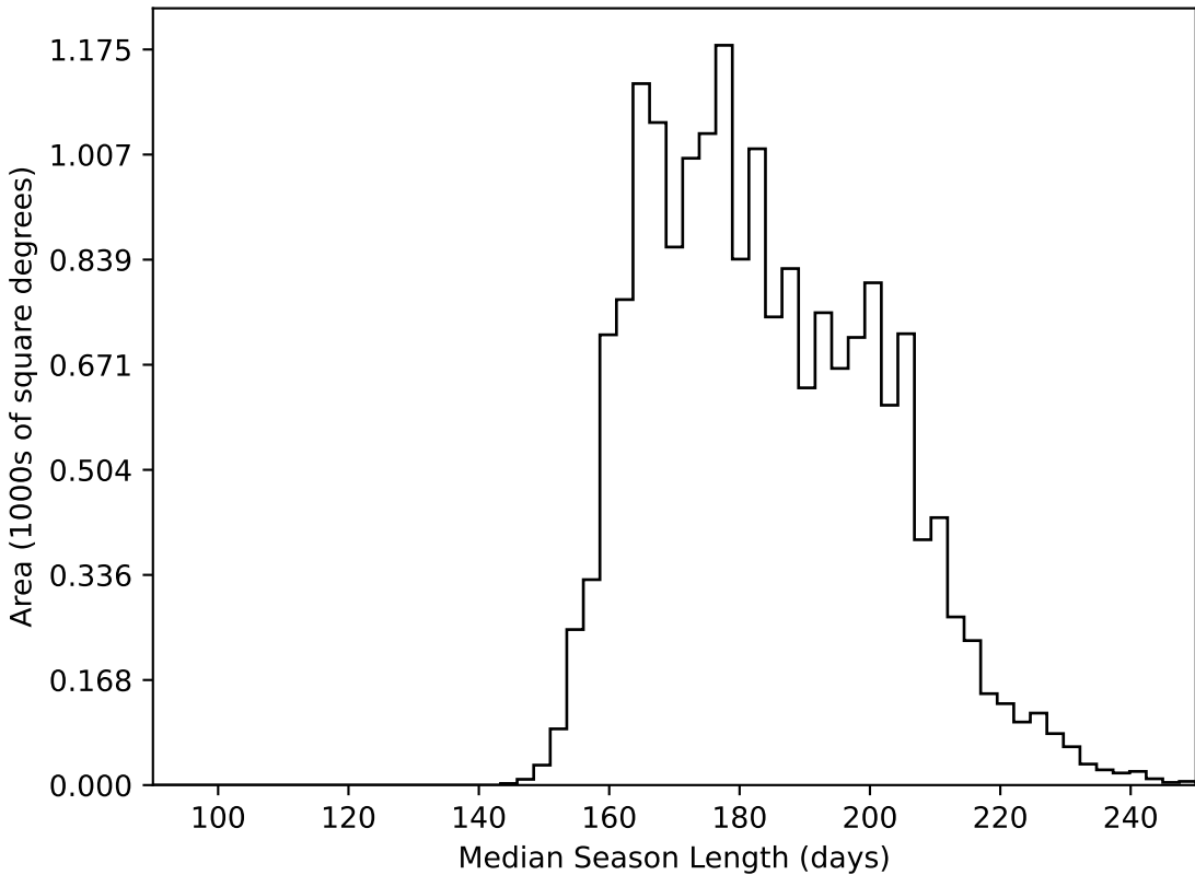
noroll_v3.4_10yrs WFD all bands: Median Season Length
