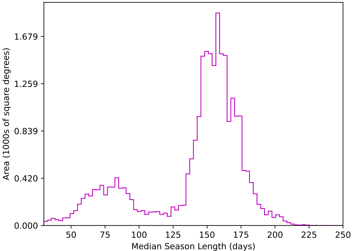
noroll_v3.4_10yrs All sky z band: Median Season Length
