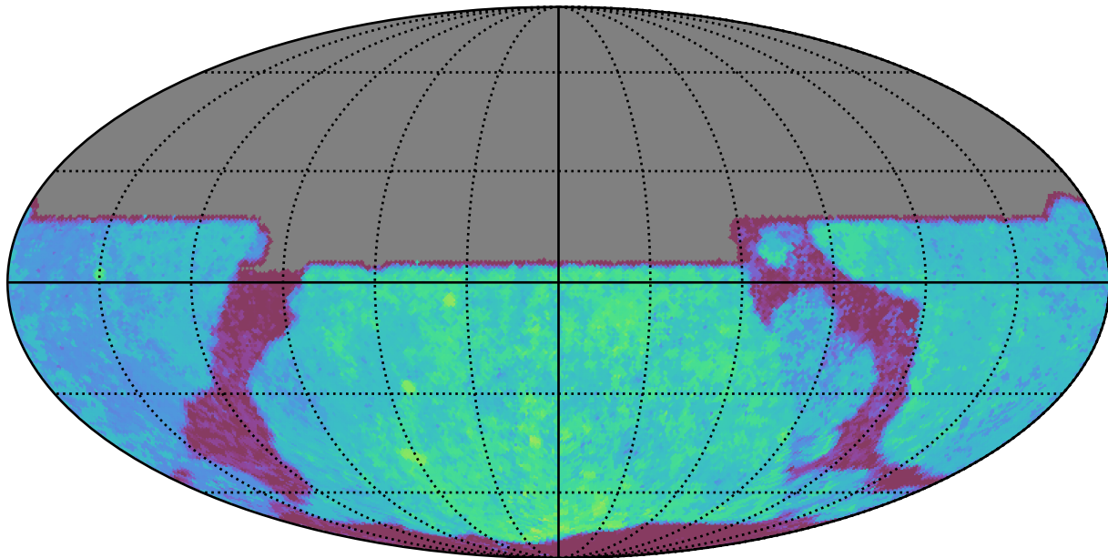
noroll_v3.4_10yrs All sky y band: Median Season Length
