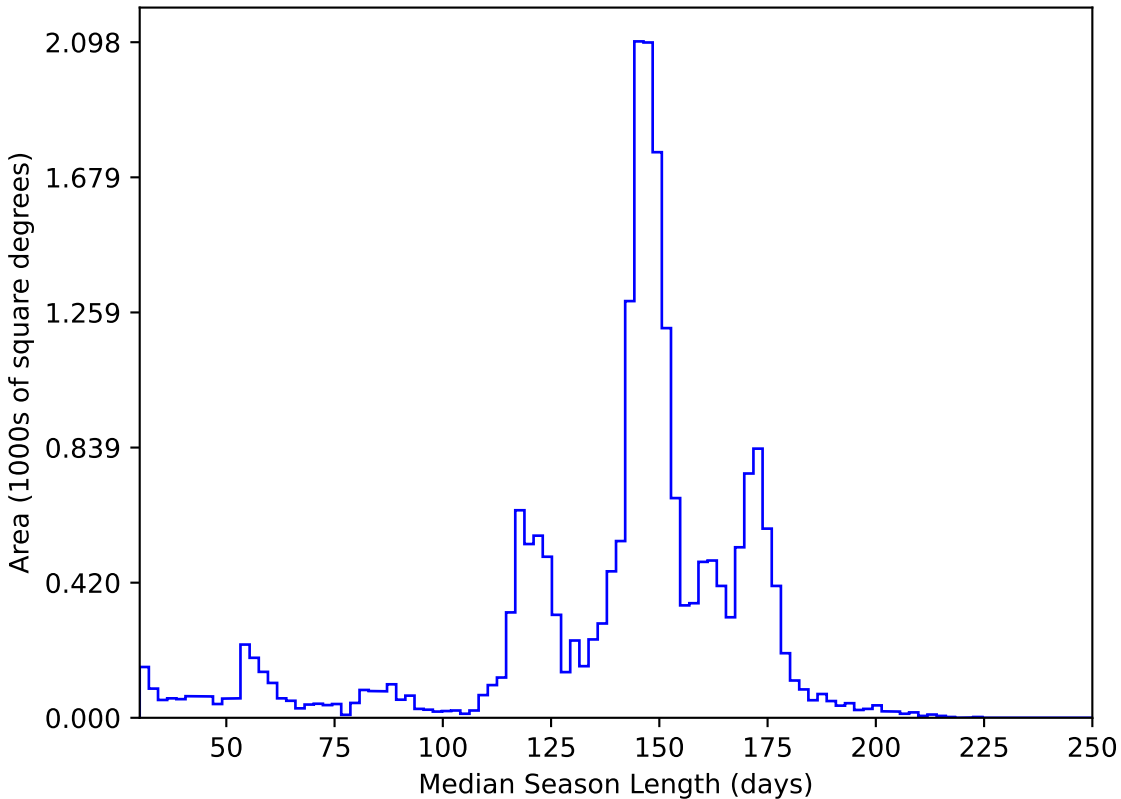
noroll_v3.4_10yrs All sky y band: Median Season Length
