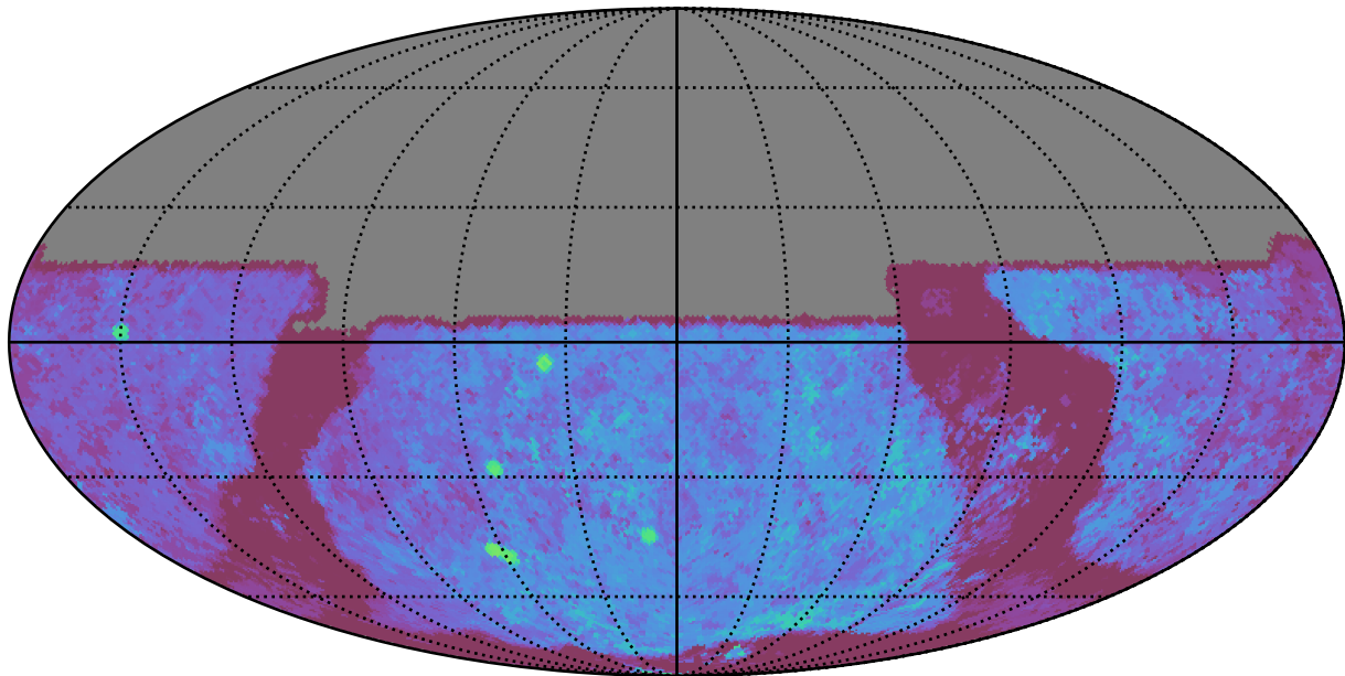
noroll_v3.4_10yrs All sky u band: Median Season Length
