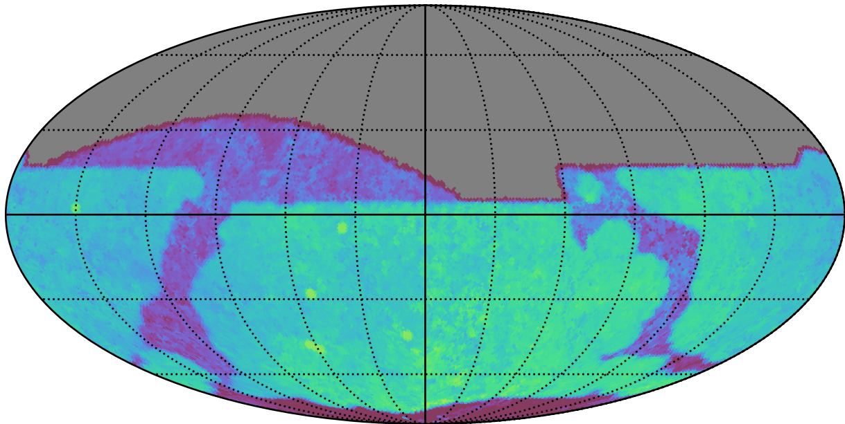
noroll_v3.4_10yrs All sky r band: Median Season Length
