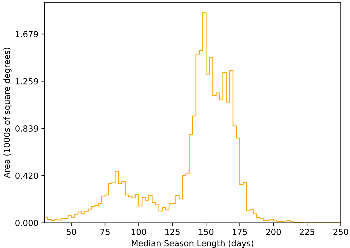
noroll_v3.4_10yrs All sky r band: Median Season Length
