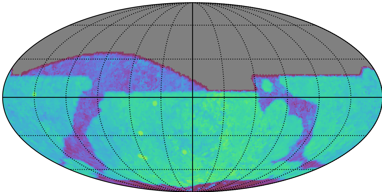
noroll_v3.4_10yrs All sky i band: Median Season Length
