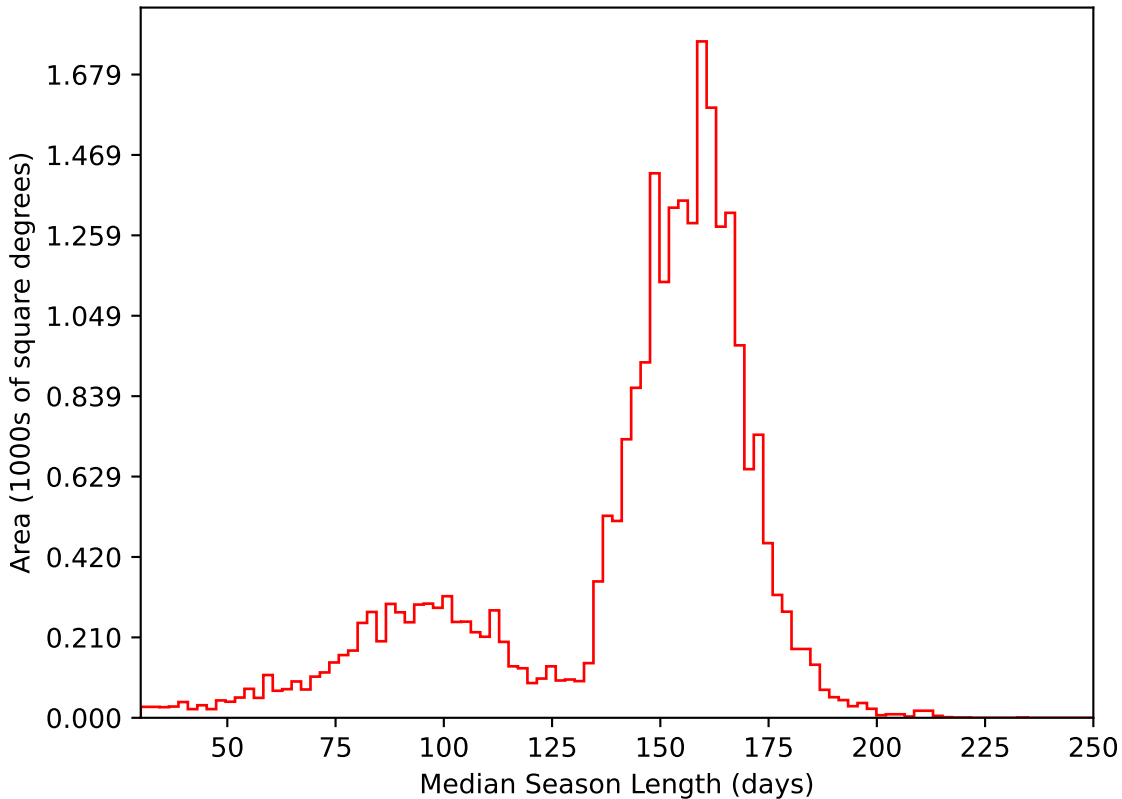
noroll_v3.4_10yrs All sky i band: Median Season Length
