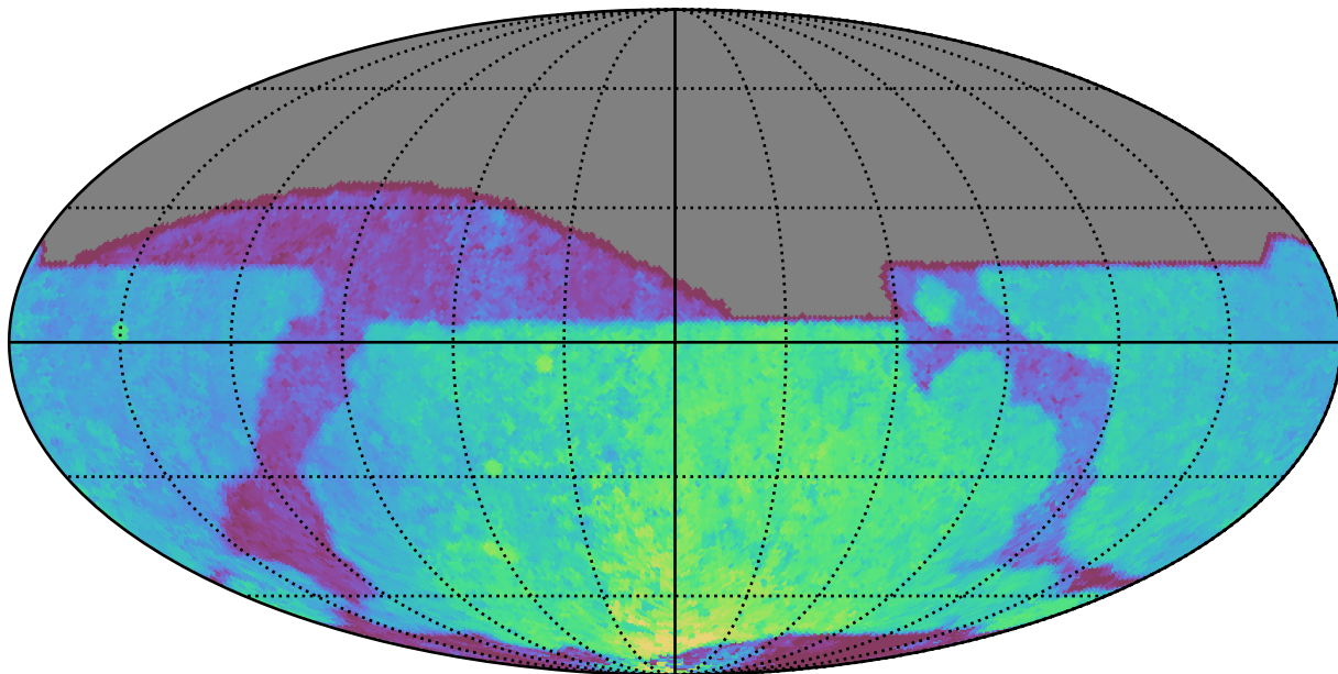
noroll_v3.4_10yrs All sky all bands: Median Season Length
