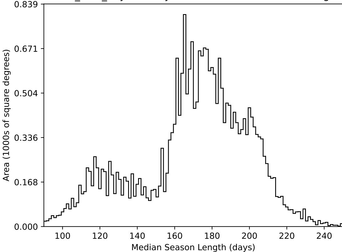
noroll_v3.4_10yrs All sky all bands: Median Season Length
