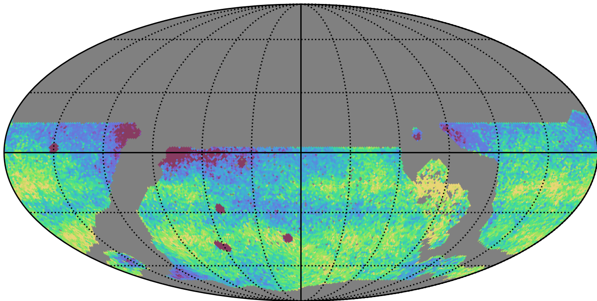
noroll_v3.4_10yrs WFD: Median Intra-Night Gap
