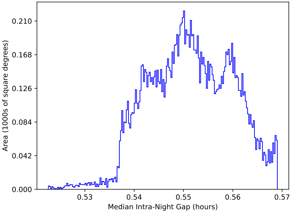
noroll_v3.4_10yrs WFD: Median Intra-Night Gap
