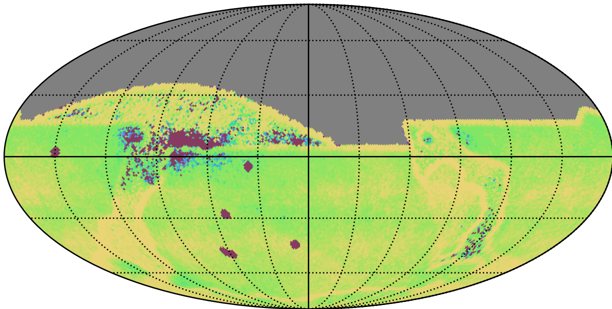
noroll_v3.4_10yrs All sky: Median Intra-Night Gap
