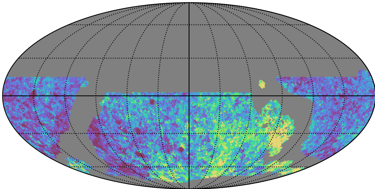
noroll_v3.4_10yrs WFD z band: Median Inter-Night Gap
