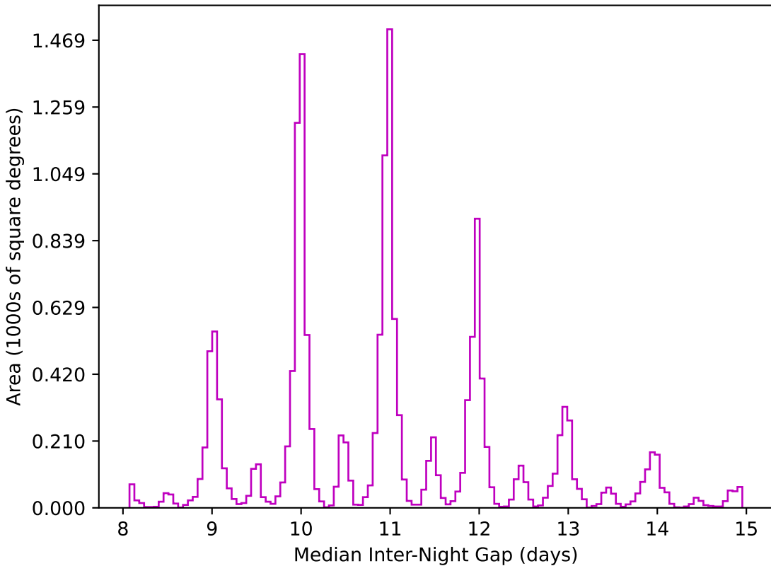
noroll_v3.4_10yrs WFD z band: Median Inter-Night Gap
