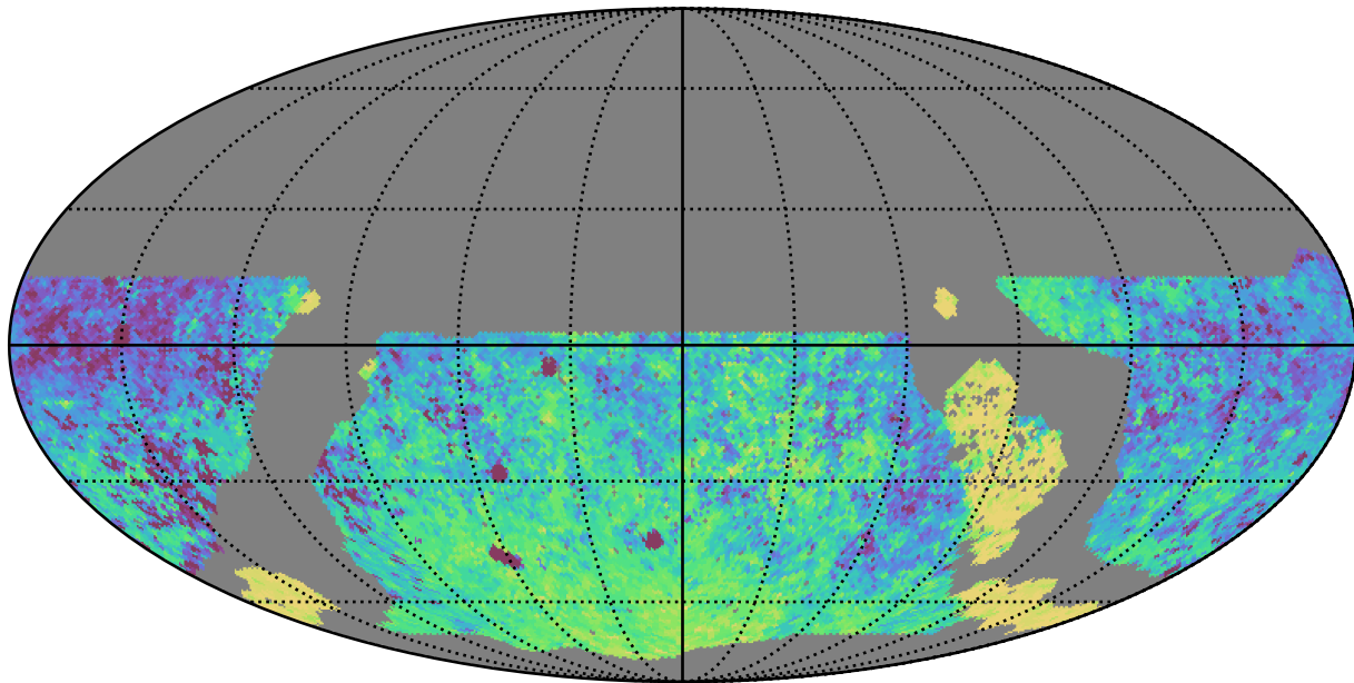
noroll_v3.4_10yrs WFD y band: Median Inter-Night Gap
