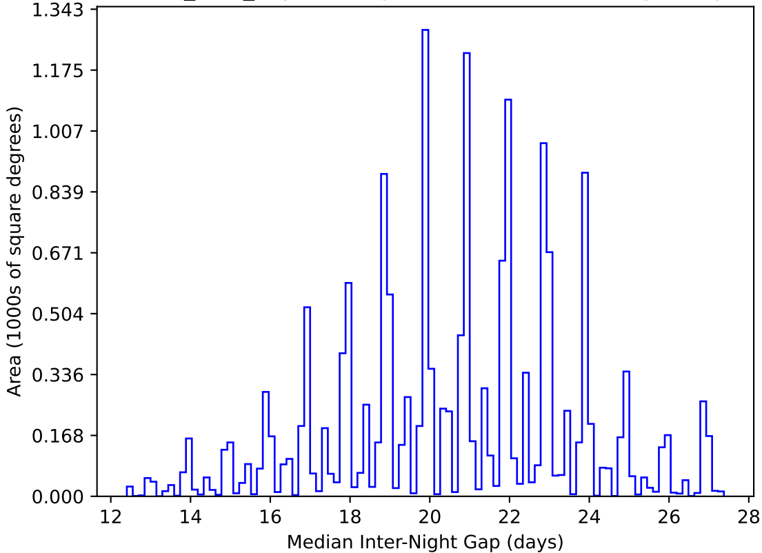
noroll_v3.4_10yrs WFD y band: Median Inter-Night Gap
