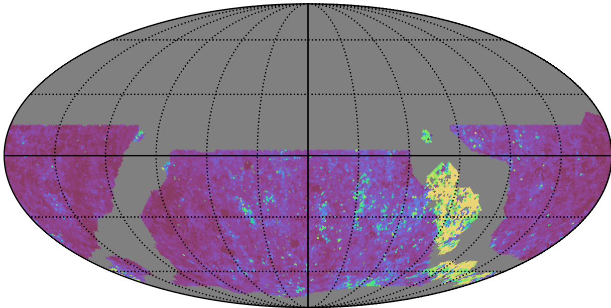
noroll_v3.4_10yrs WFD u band: Median Inter-Night Gap
