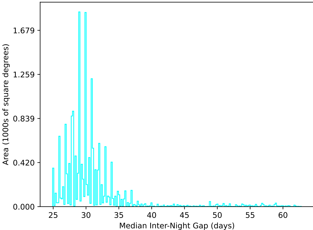
noroll_v3.4_10yrs WFD u band: Median Inter-Night Gap
