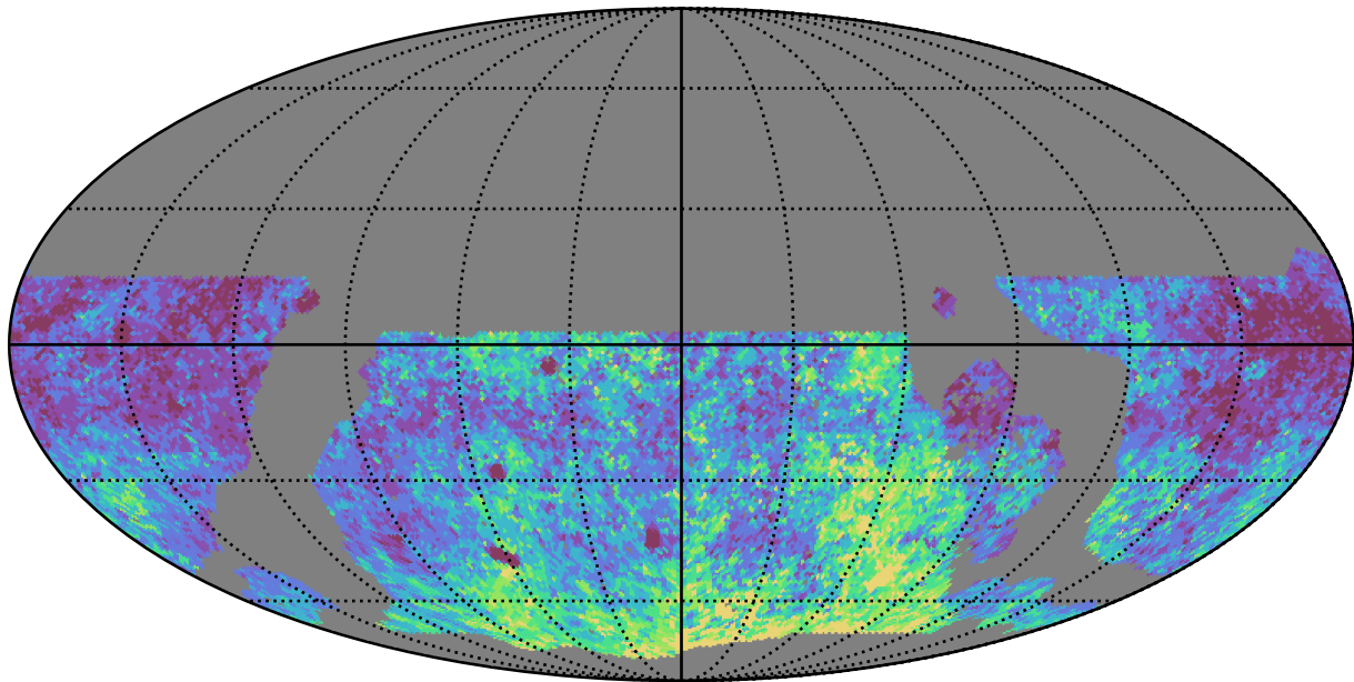
noroll_v3.4_10yrs WFD r band: Median Inter-Night Gap
