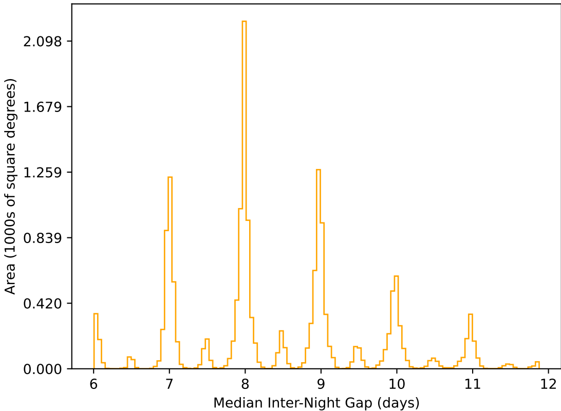
noroll_v3.4_10yrs WFD r band: Median Inter-Night Gap
