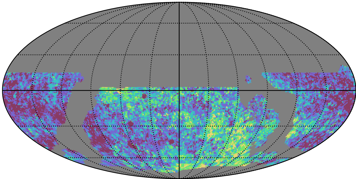
noroll_v3.4_10yrs WFD i band: Median Inter-Night Gap
