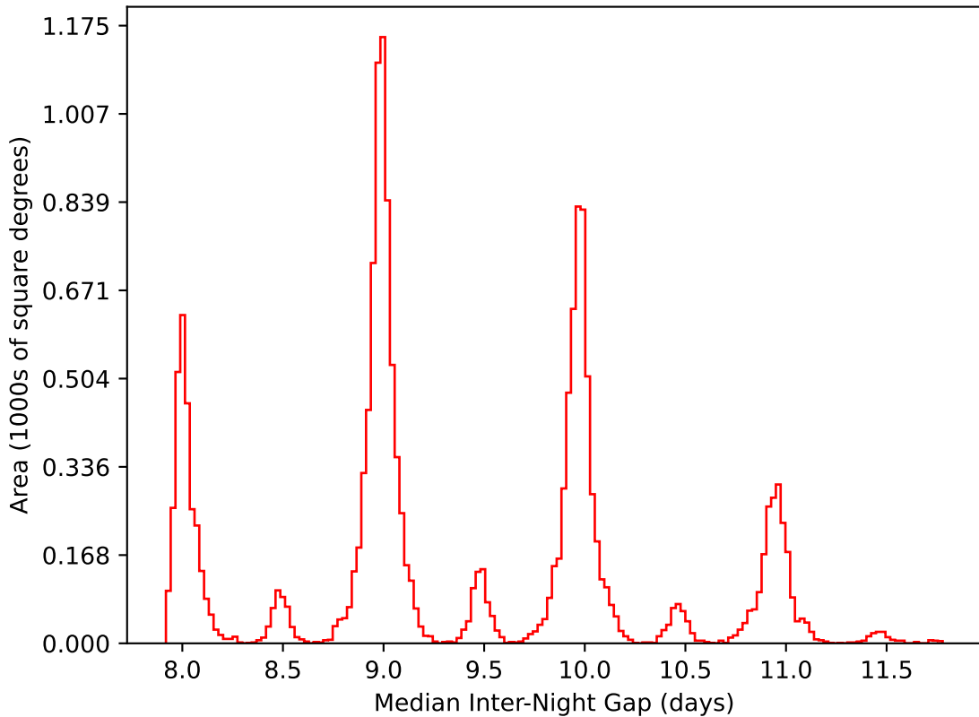
noroll_v3.4_10yrs WFD i band: Median Inter-Night Gap
