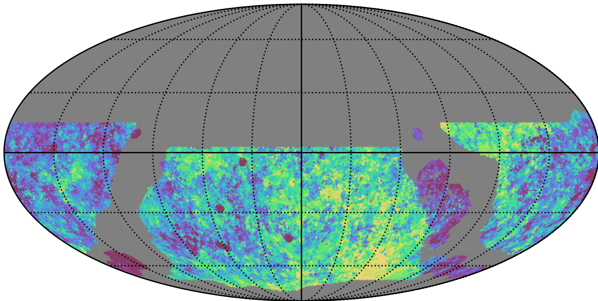
noroll_v3.4_10yrs WFD g band: Median Inter-Night Gap
