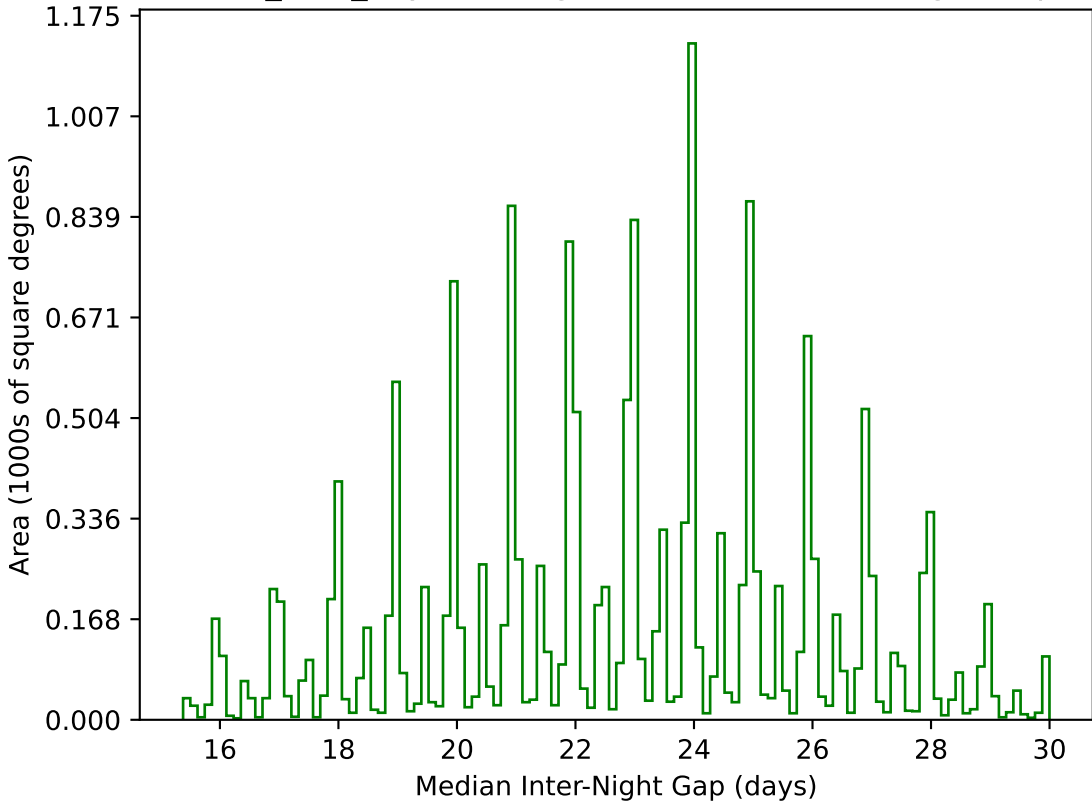
noroll_v3.4_10yrs WFD g band: Median Inter-Night Gap
