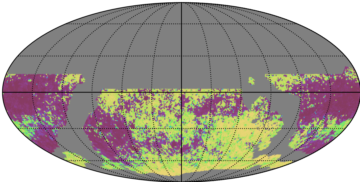
noroll_v3.4_10yrs WFD all bands: Median Inter-Night Gap
