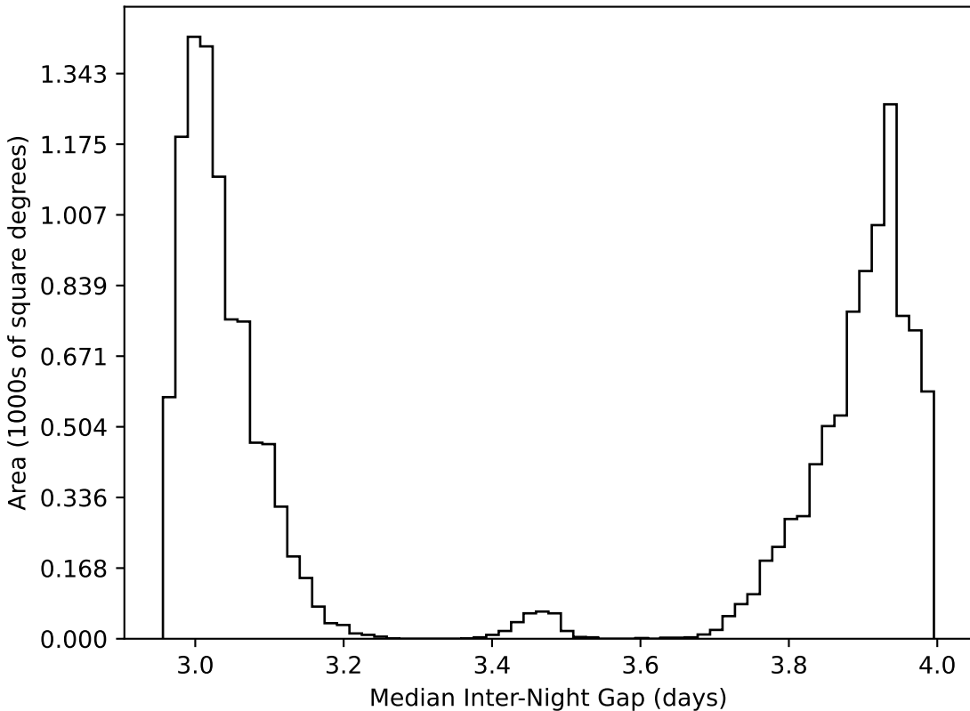
noroll_v3.4_10yrs WFD all bands: Median Inter-Night Gap
