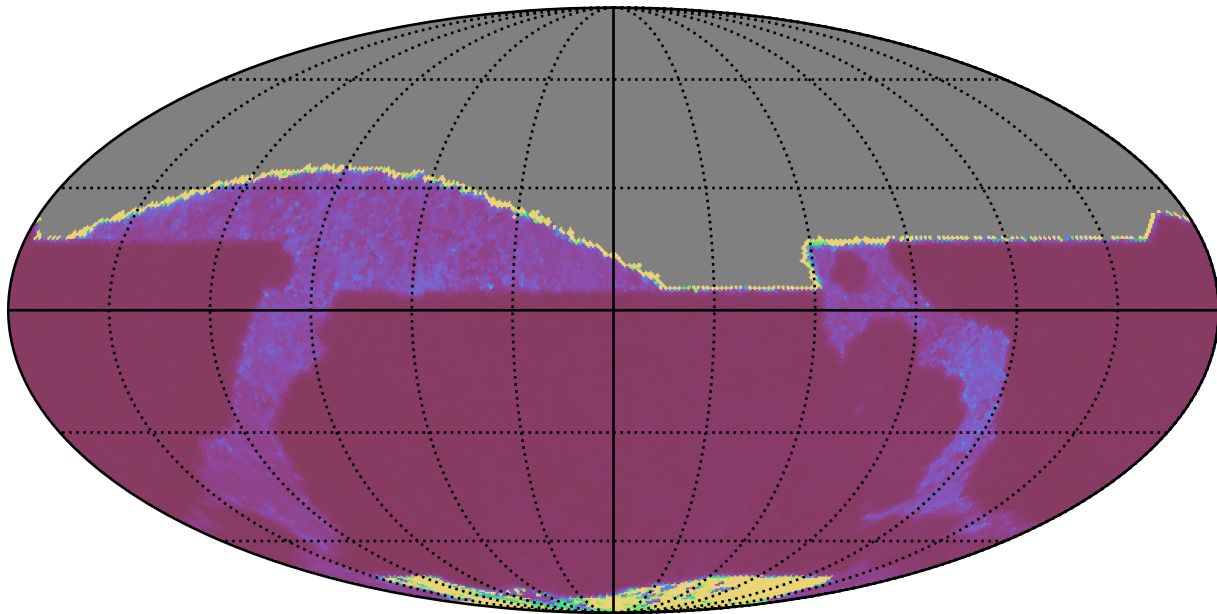
noroll_v3.4_10yrs All sky z band: Median Inter-Night Gap
