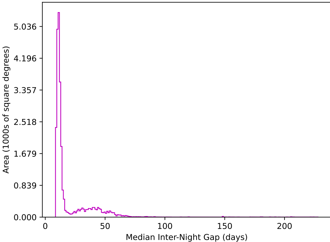
noroll_v3.4_10yrs All sky z band: Median Inter-Night Gap
