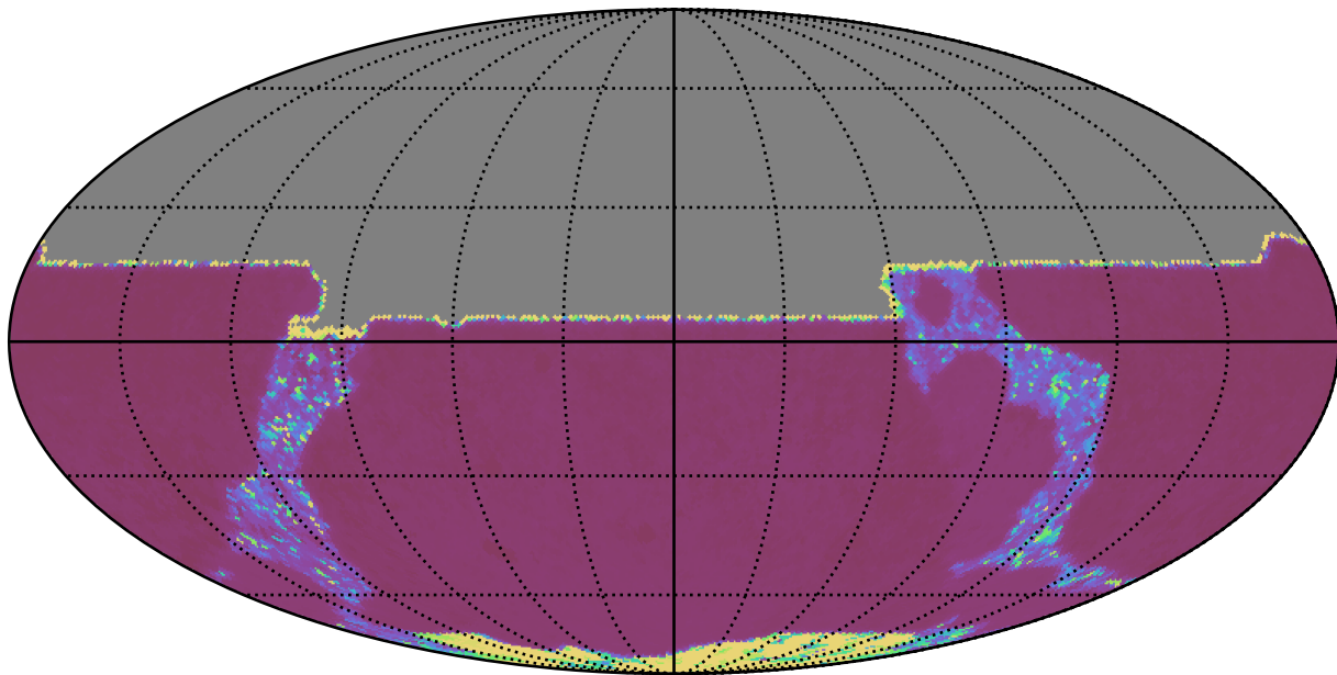
noroll_v3.4_10yrs All sky y band: Median Inter-Night Gap
