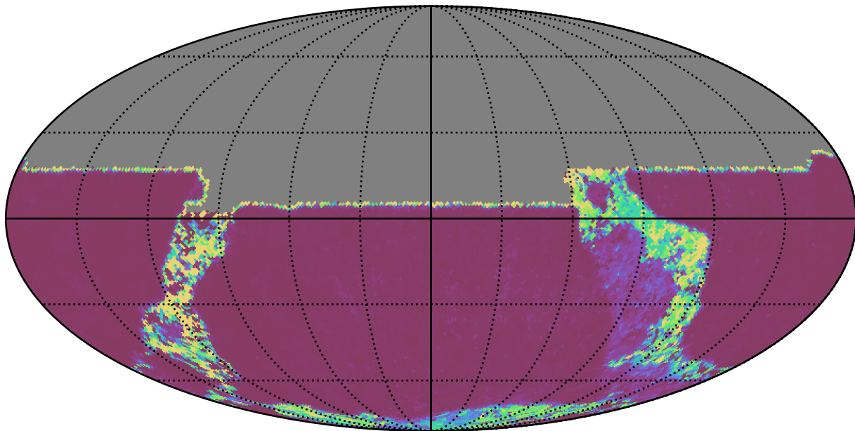
noroll_v3.4_10yrs All sky u band: Median Inter-Night Gap
