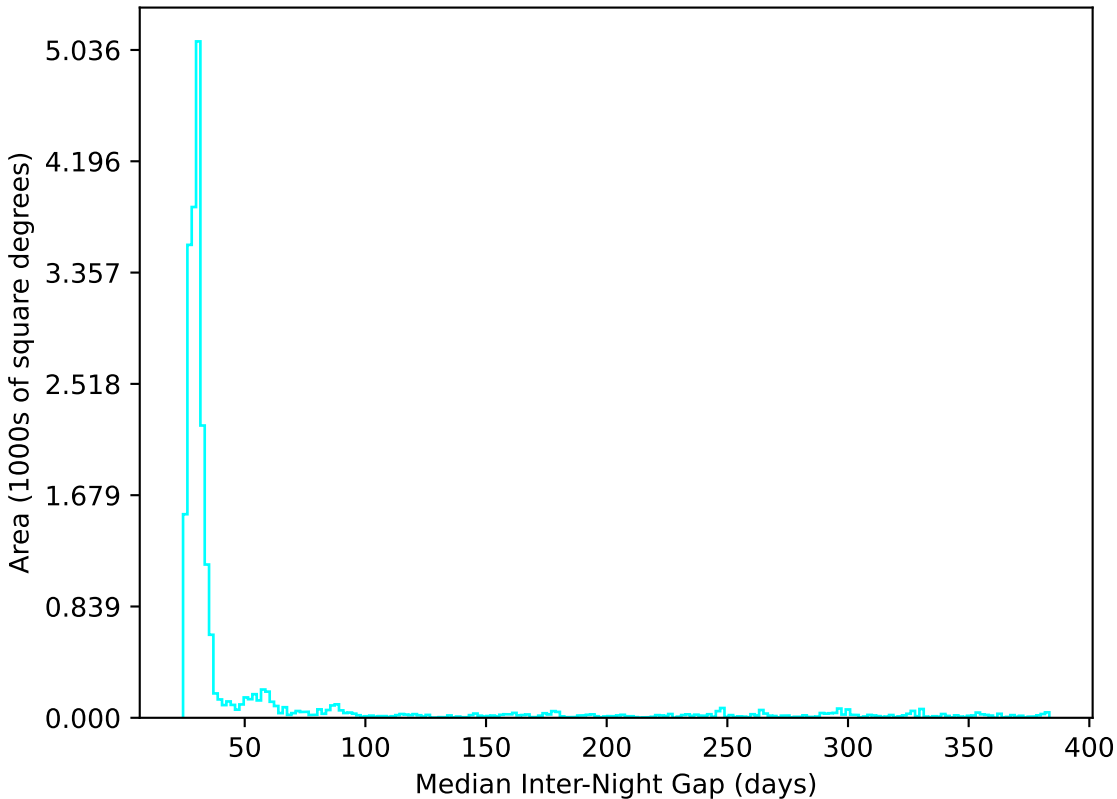
noroll_v3.4_10yrs All sky u band: Median Inter-Night Gap
