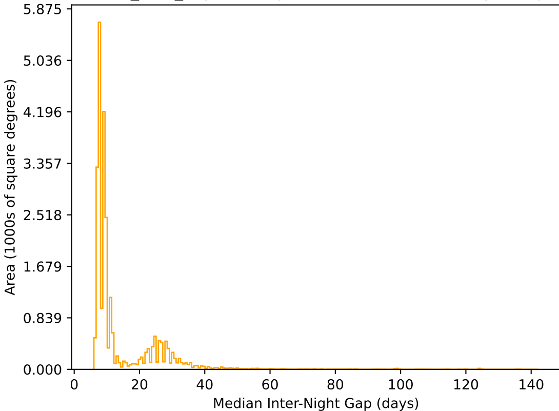
noroll_v3.4_10yrs All sky r band: Median Inter-Night Gap
