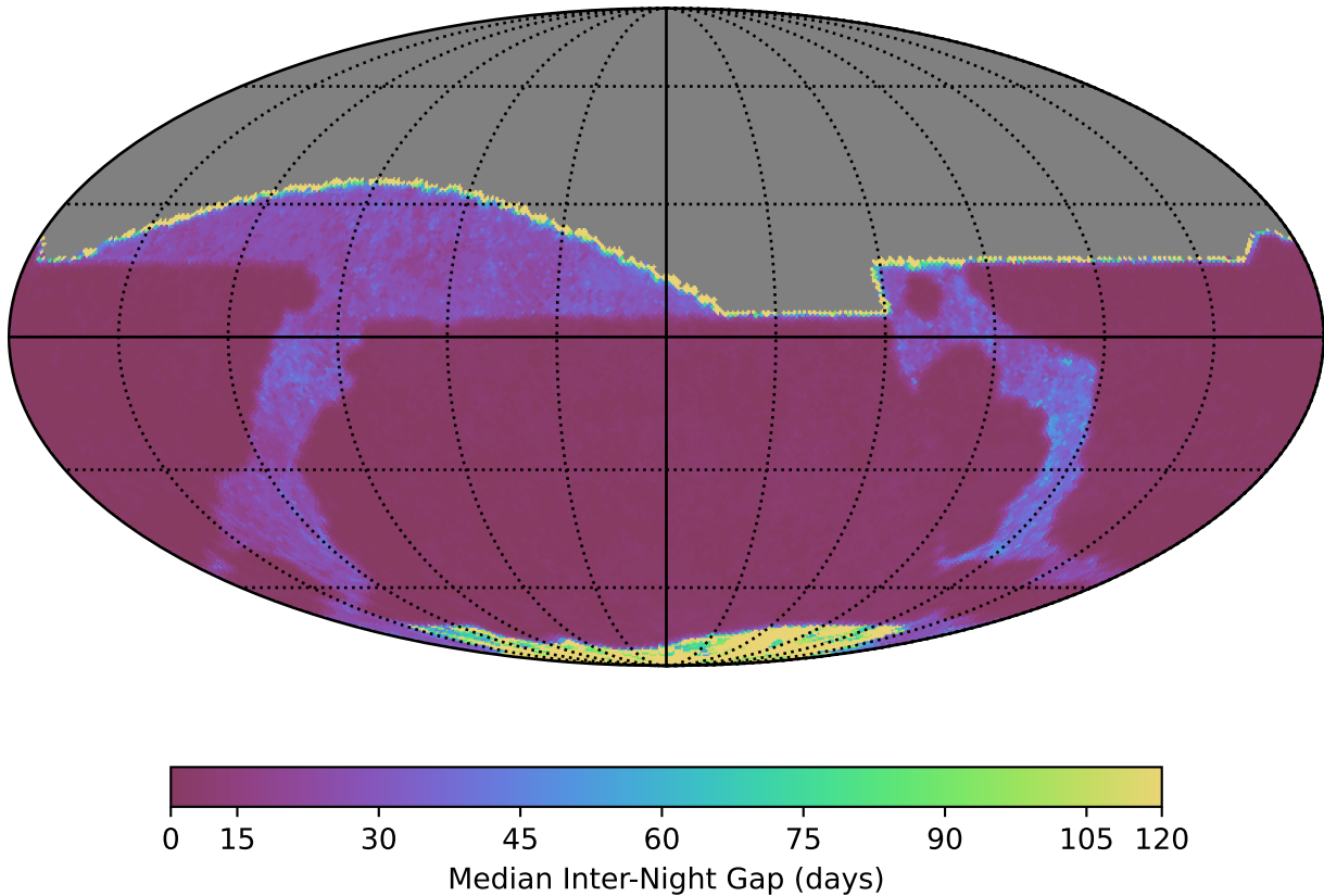
noroll_v3.4_10yrs All sky i band: Median Inter-Night Gap
